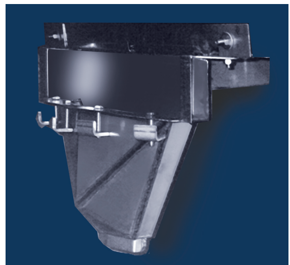
SUPERFLUX® trays with PURGE downcomer option resist fouling in very severe applications.
