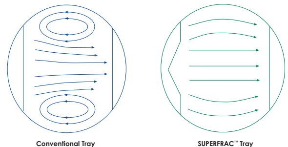
Liquid flow distribution comparison between conventional trays with truncated downcomers and a multi-chordal SUPERFRAC® tray.
