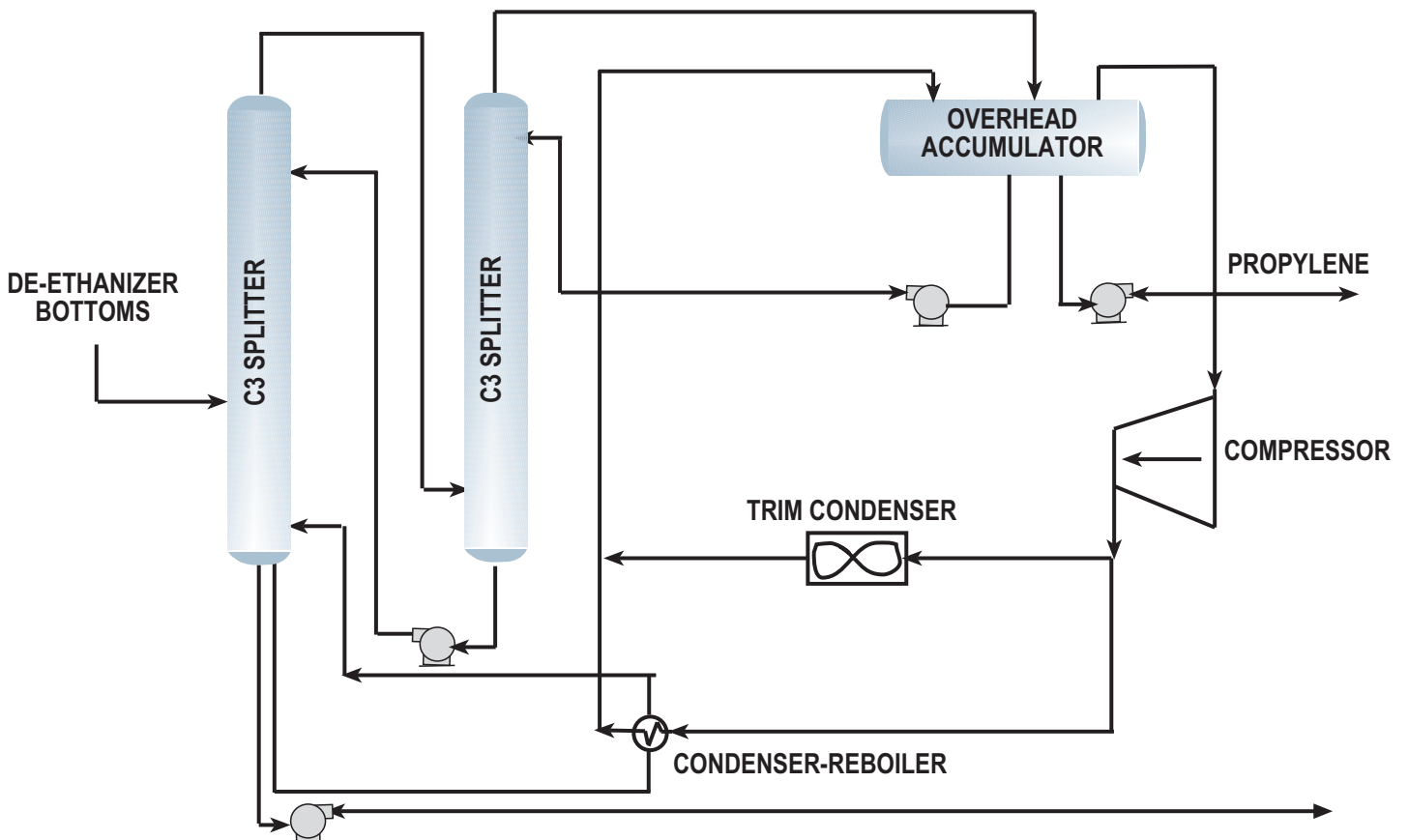
C 3 Splitter Simplified Process Flow Diagram
