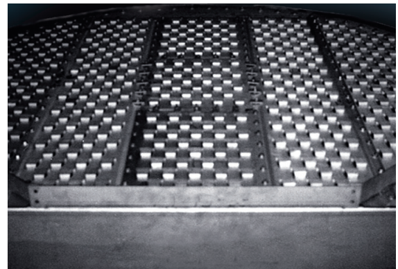
PROVALVE® Valves
