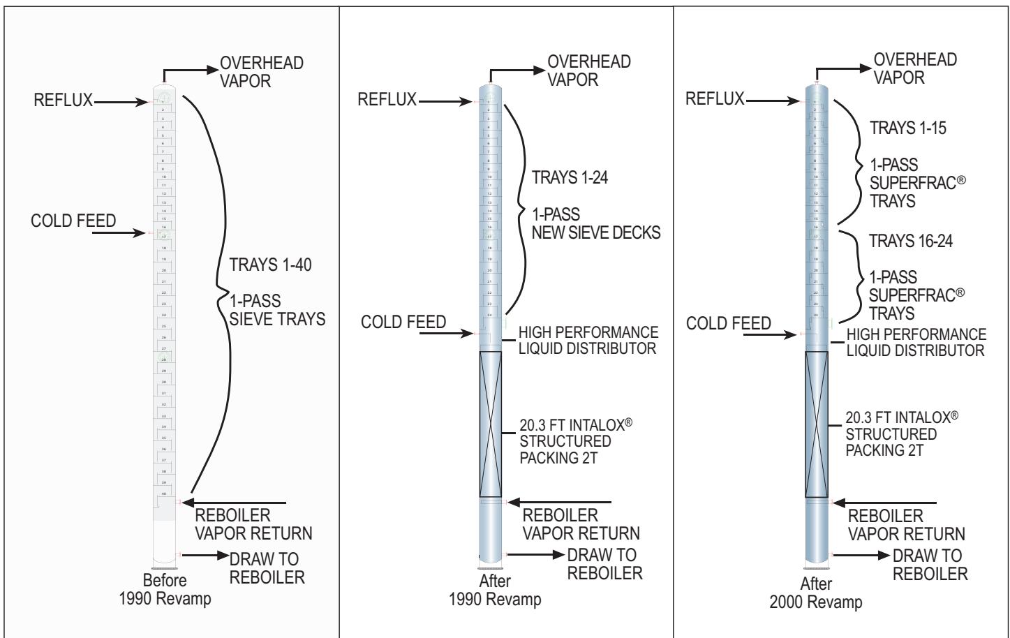
Column Layouts Before and After Revamps
