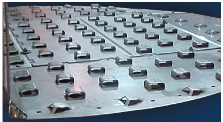
SUPERFLUX® Tray for Bioethanol Beer Stripper
