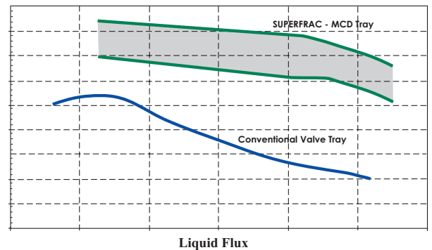
Capacity gains for SUPERFRAC® trays can be substantial while still maintaining high efficiencies.
