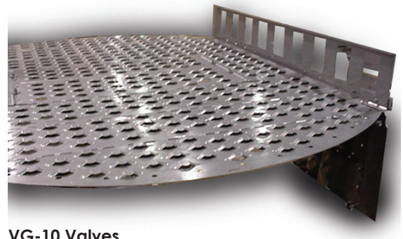
VG-10 Valves
