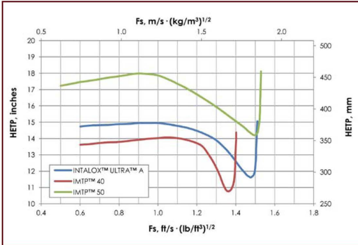
Light hydrocarbon distillation at 83 psia [5.73 barA] pressure.
