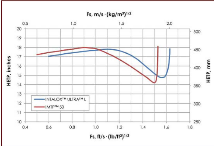
Light hydrocarbon distillation at 83 psia [5.73 barA] pressure.
