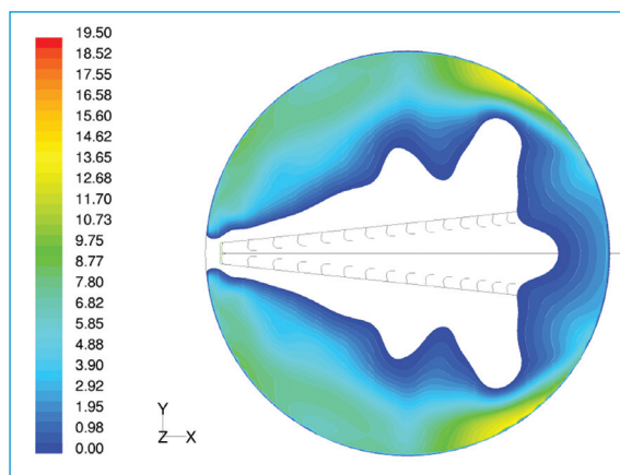
Model 768 YORK-EVENFLOW vane inlet device.
