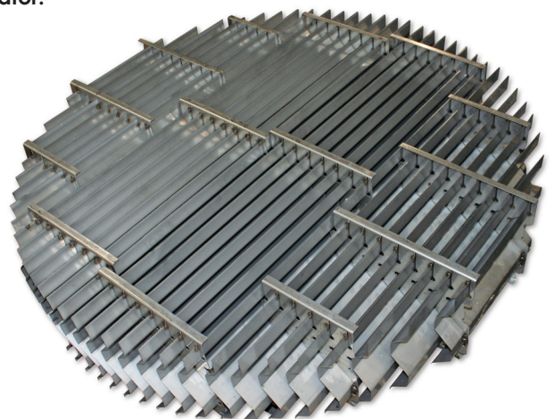
FLEXICHEVRON® style VIII mist eliminator in metal.
