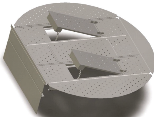
Explosion doors can provide protection to trays during an upset.
