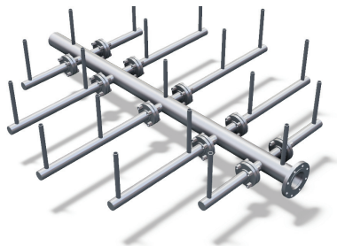
Spray distributor for FLEXICHEVRON® mist eliminator.
