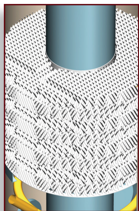
KFBE packing.
