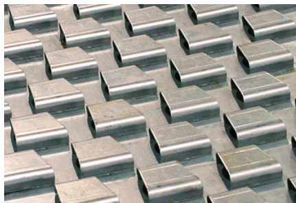
PROVALVE® tray.
