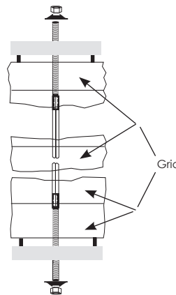
Through rod.
