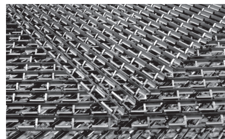
GLITSCH-GRID EF-25A grid packing.
