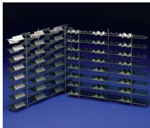
FLEXIGRID® severe service grid packing. Style 3-45 (left). Style 2-45 (right).
