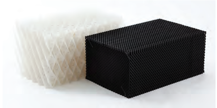
FLEXIPAC® 2Y structured packing in polypropylene (white) and FLEXIPAC® 500Z HC® structured packing in PFA (black).
