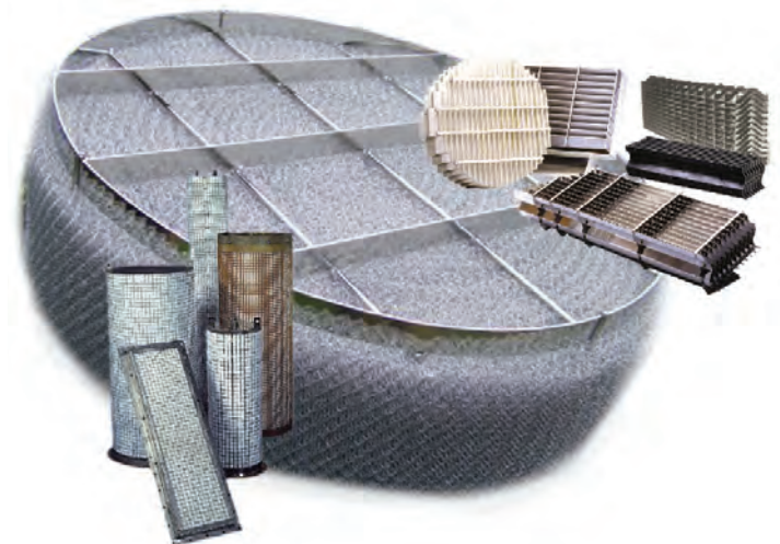
Left (FLEXIFIBER® mist eliminators), center (DEMISTER® mist eliminators), and right (FLEXICHEVRON® mist eliminators).
